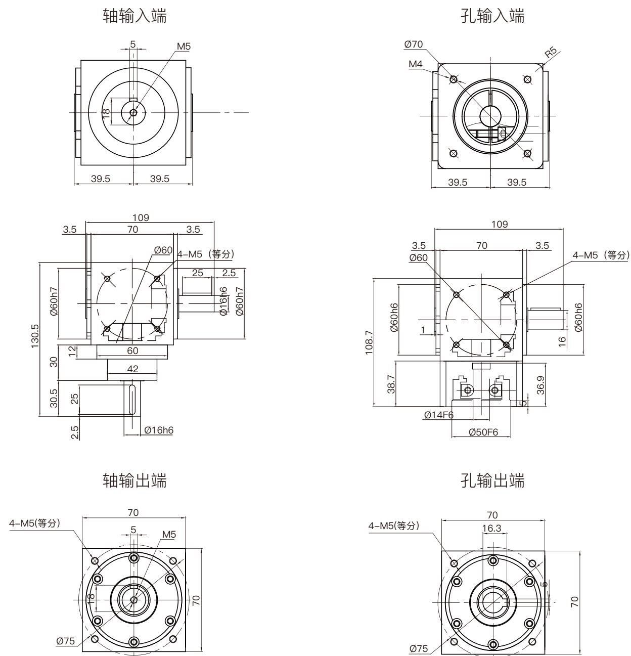
ZQH70-1外形图 / ZQH70-1 Outline Drawing
