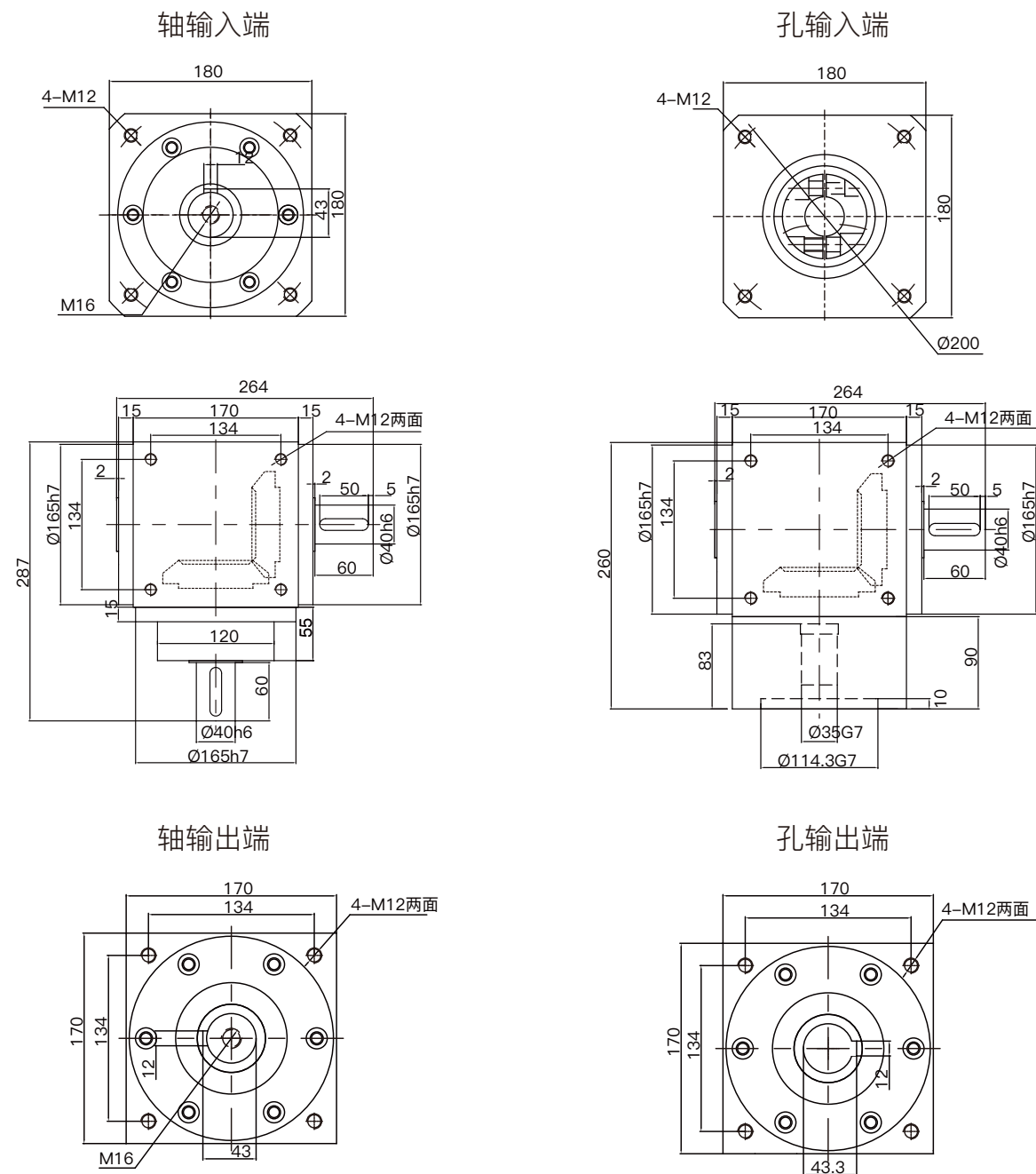
ZQH170-1外形图 / ZQH170-1 Outline Drawing
