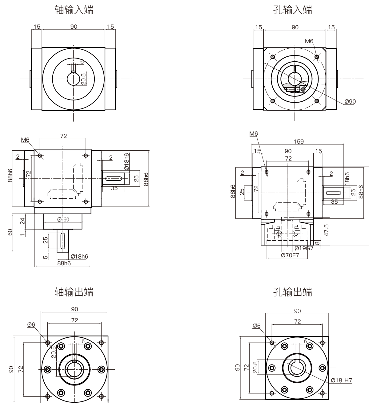
ZQH90-1外形图 / ZQH90-1 Outline Drawing
