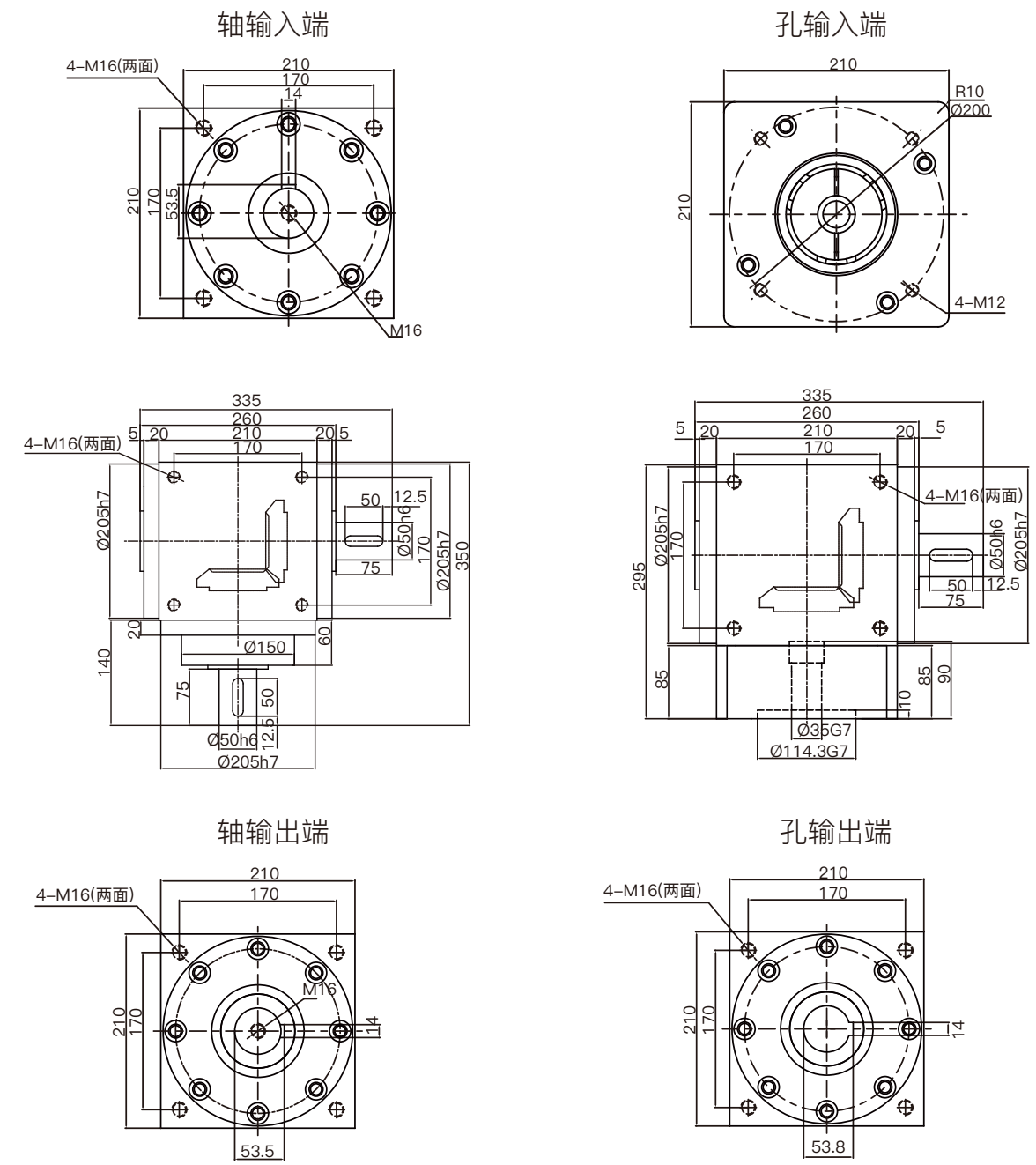
ZQH210-1外形图 / ZQH210-1 Outline Drawing
