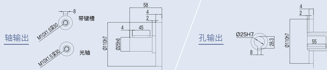
输出方式图形/Output Method Graph
