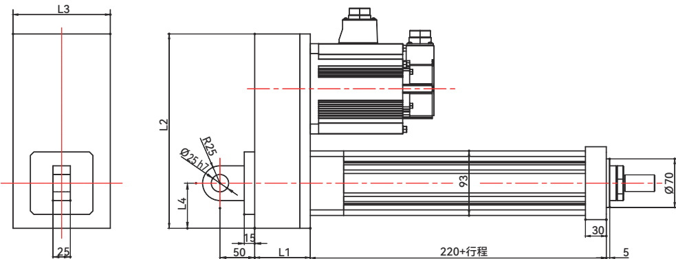
M5:尾部单耳轴
